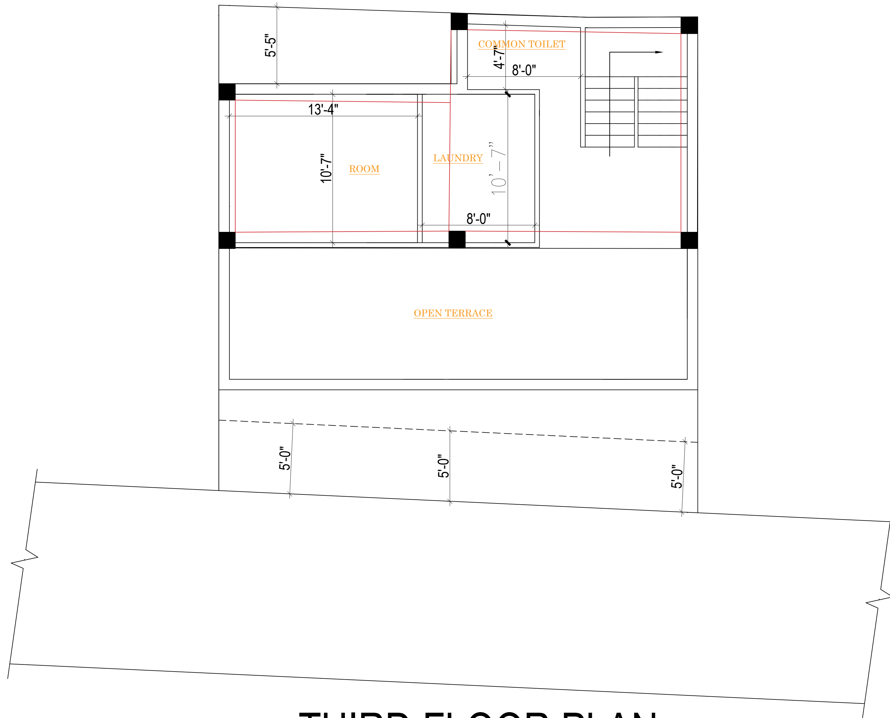
THIRD FLOOR PLAN AREA=483 SQ.FT
